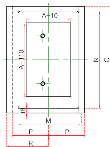
D-D VIEW
